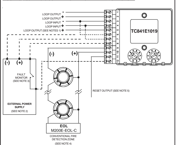
FIGURE 3: TC841E1019 CONVENTIONAL ZONE INTERFACE MODULE
